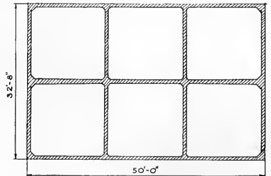
SECTION D-D. HORIZONTAL SECTION THROUGH BIN WALLS
